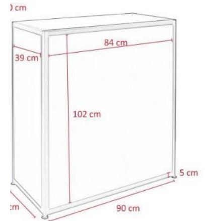
Counter with storage White @97 € Dimensions : L 90 x P 50 x H 110 Usable surface area (for print cover) : L 84 x H 102
